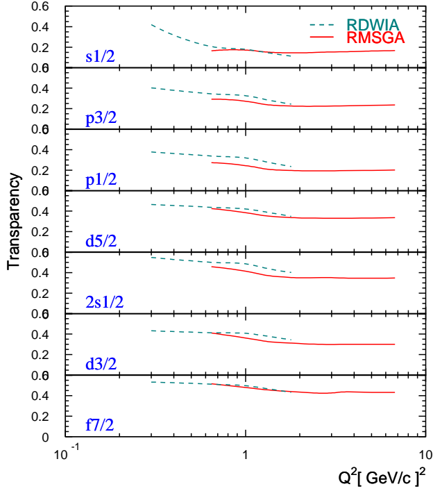
Figure 1. The Q^2 dependence of the computed nuclear transparency for the proton levels in ^{56}\text{Fe} as obtained in the RDWIA (dashed line) and RMSGA (solid line) approach.
