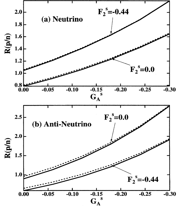
FIG. 8. (a) Ratios of integrated proton-to-neutron quasielastic yield for the ^{12}\text{C}(\nu, \nu'N) reaction as functions of G_A^s for two values of strange magnetic form factor F_2^s . In each case, the dashed line is the impulse approximation result while the solid line has been corrected for meson exchange currents. The incident neutrino energy is assumed to be 200 MeV for both cases and the range of integration was chosen to be 50 \leq T_F \leq 120 \text{ MeV} to simulate the LSND experiment [22]. (b) Same as in (a) but for antineutrino scattering.
