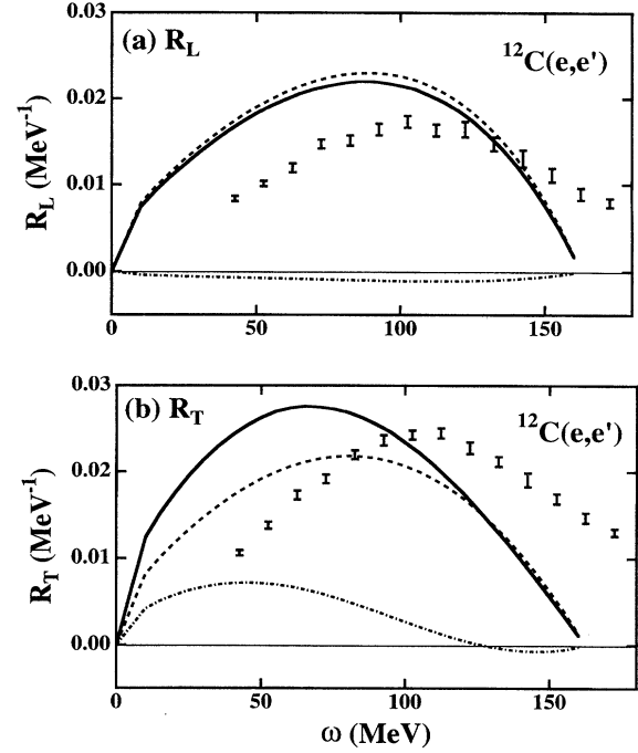
FIG. 1. (a) Longitudinal, R_L , and (b) transverse, R_T , response functions for the ^{12}\text{C}(e, e') reaction plotted against the energy transfer \omega . The three momentum transfer involved in the inclusive reaction is |\vec{k}| = 400 MeV. A RFG model without any binding energy corrections ( B=0 ) and with a Fermi momentum of k_F = 225 MeV was used to calculate the response functions. Experimental data, taken from [50], are shown for reference but no attempt to fit the data by varying B and k_F has been made. The dashed line represents the impulse approximation results while response functions obtained with soft-pion MEC corrections are shown with solid lines. Also shown in the figures using the dash-dotted lines are the individual contributions from soft-pion two-body currents.
