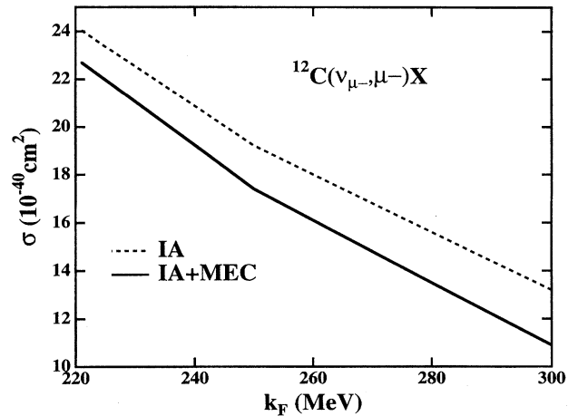
FIG. 2. ^{12}\text{C}(\nu_{\mu^-}, \mu^-)X total cross section obtained by folding the LSND neutrino flux [30] vs the Fermi momentum k_F . The dashed curve is the impulse approximation result while the solid curve is obtained with the soft-pion MEC corrections using the RFG model of the nucleus with no binding energy correction ( B=0 ). For k_F = 225 MeV, which is the usual value used for ^{12}\text{C} , the total cross section is reduced from 24 to 22.7 ( \times 10^{-40} cm ^2 ) when corrected for two-body current effects.
