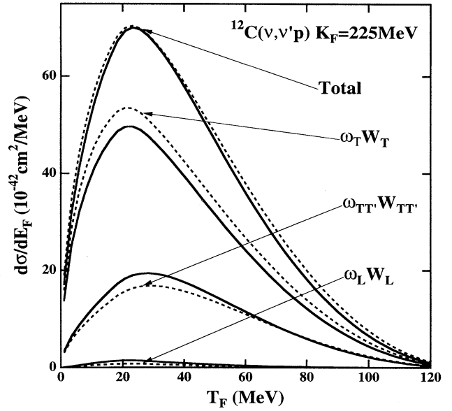
FIG. 6. Various structure function contributions to the ^{12}\text{C}(\nu, \nu'p) differential cross section shown in Fig. 5. Both the impulse approximation and MEC corrected results for the transverse, \omega_T W_T , longitudinal, \omega_L W_L , and transverse-transverse, \omega_{TT'} W_{TT'} , contributions are shown explicitly using the dashed and solid lines, respectively. Note that the two-body corrected contributions from the transverse and transverse-transverse contributions cancel leading to a small overall MEC correction to the impulse approximation. For antineutrino scattering the transverse-transverse contribution changes sign resulting in a smaller differential cross section but in a larger MEC effect compared to neutrino scattering.
