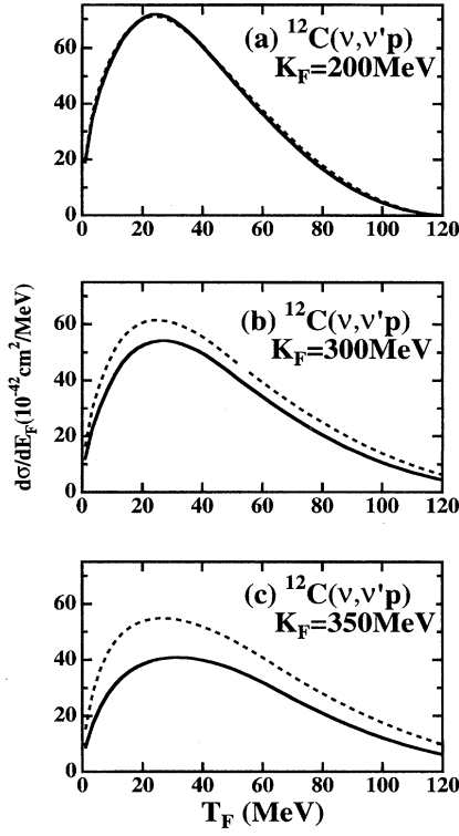
FIG. 4. ^{12}\text{C}(\nu, \nu' p) differential cross section vs the kinetic energy of the ejected nucleon, T_F , for (a) k_F = 200 MeV, (b) k_F = 300 MeV, and (c) k_F = 350 MeV. The incident neutrino energy is assumed to be 200 MeV while the values for the strange quark form factors used are F_2^s = -0.21 and G_A^s = -0.19 . The long dashed curve is the impulse approximation result while the solid curves have been obtained with soft-pion MEC corrections.
