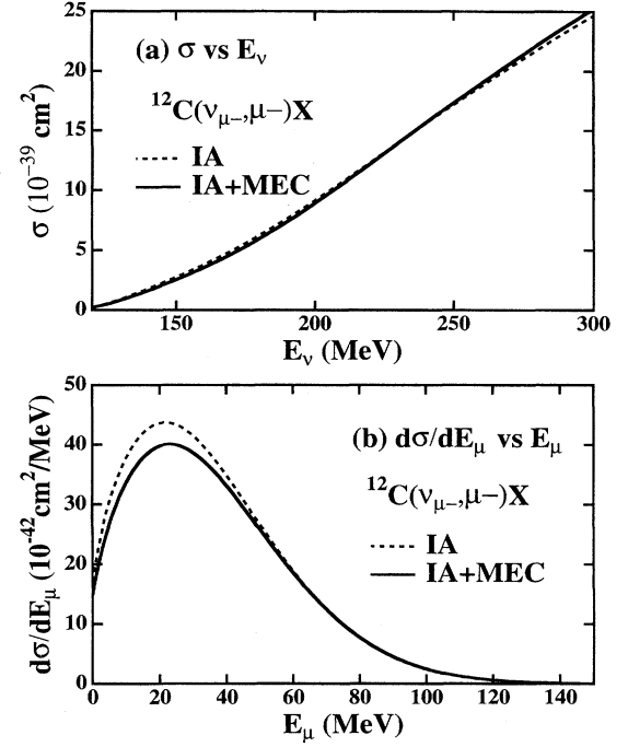
FIG. 3. (a) ^{12}\text{C}(\nu_{\mu^-}, \mu^-)X total cross section as a function of incoming neutrino energy E_\nu taking into account the Coulomb correction for the outgoing muon. As in Fig. 2, the RFG model is used to model the nucleus with k_F = 225 MeV and B=0 . The dashed line is the impulse approximation result while the solid line includes two-body soft-pion MEC effects. Note that in this particular case there is very little difference between the two results. (b) Differential cross section d\sigma/dE_\mu for the same process obtained with and without the soft-pion MEC correction plotted against the outgoing muon kinetic energy E_\mu . The results for this figure are obtained by folding the LSND neutrino energy distribution obtained from [30].
