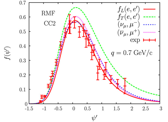
Fig. 4. (Color online.) Longitudinal and transverse scaling functions for (e, e') compared with f(\psi') evaluated from (\nu, \mu^-) and (\bar{\nu}, \mu^+) . All results have been evaluated with the RMF approach using the CC2 current operator. The kinematics selected correspond to fixed values of the incident lepton energy, \varepsilon = 1 GeV, and momentum transfer, q = 0.7 GeV/c. The averaged experimental function extracted from longitudinal electron scattering data is also shown [4].
